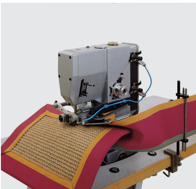
View of the TITAN DK3700C sewing large tape of 150 mm width on a sisal carpet.
