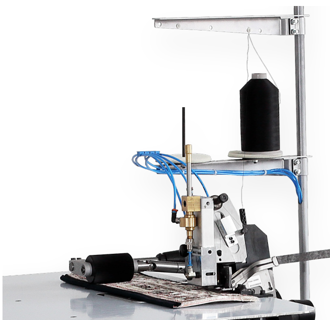
Three threads stitch
